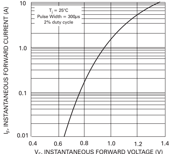
Fig. 2 Typ Forward Characteristics (per element)
