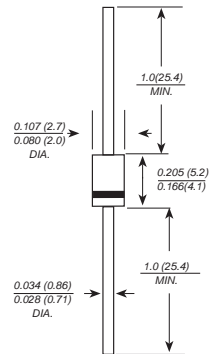
DO-41
