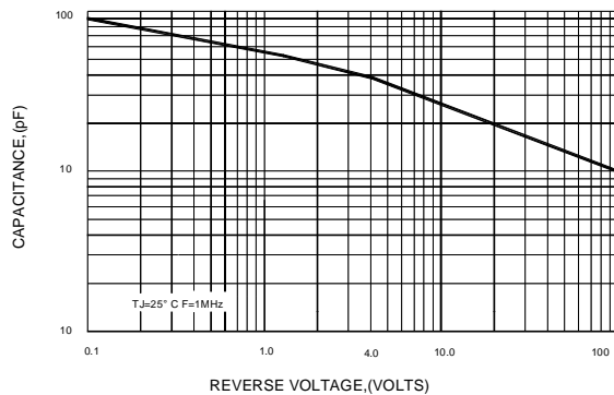
FIG.5-TYPICAL JUNCTION CAPACITANCE
